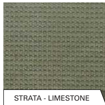
STRATA - LIMESTONE
