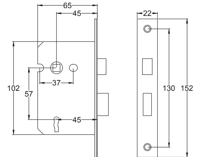
3 Lever Sash Lock
