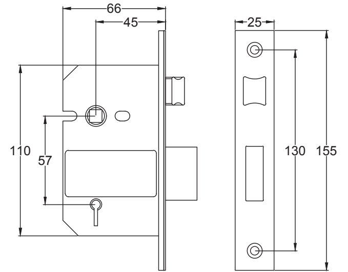
5 Lever Sash Lock
