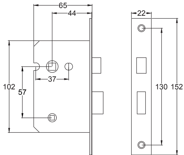
Bathroom Sash Lock
