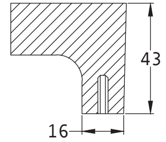
Section x-x
