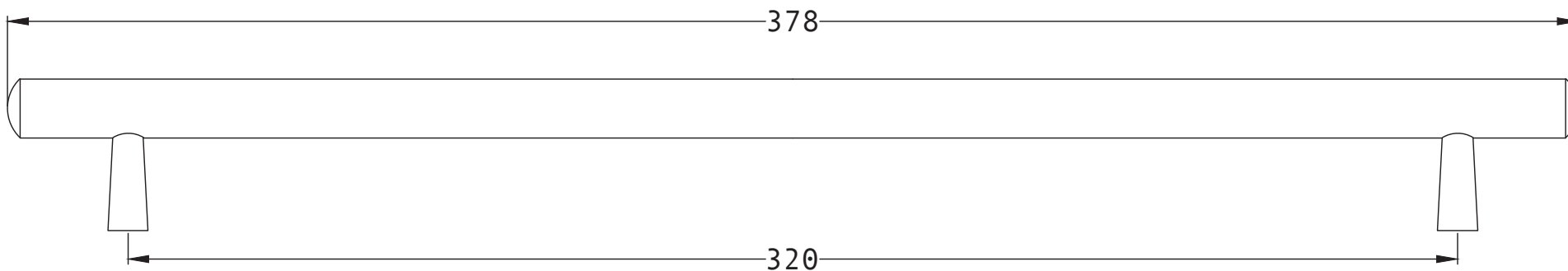
T-Bar Tilaa Cabinet Pull Handle W7763-320
