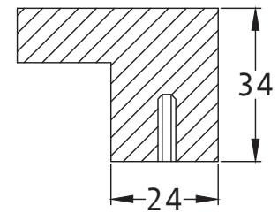
Section x-x
