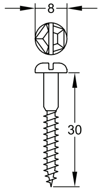
4 x 30mm PY4X30
