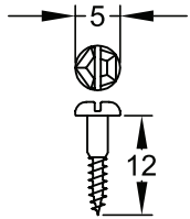
2.5 x 12mm PY2.5X12
