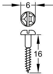
3 x 16mm PY3X16
