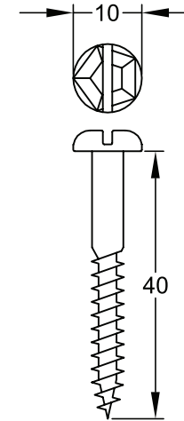
5 x 40mm PY5X40
