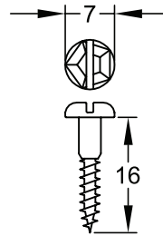
3.5 x 16mm PY3.5X16
