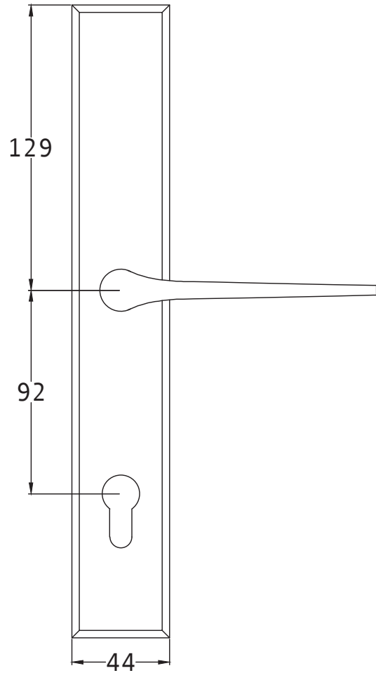
Gio LH Door Handle on Plate MP4189.LH
