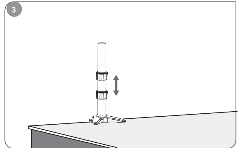
Adjust locating ring at proper height and screw up tight to hold the mount.
