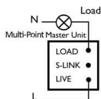
Fig 1. Wiring for 1-Way Circuits
