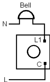
One way circuit
