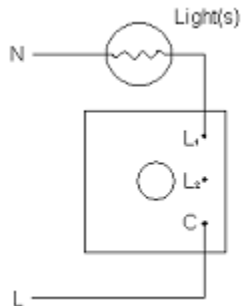
One way circuit
