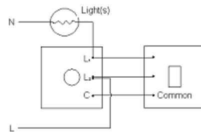
Two-way circuit (type 2)
