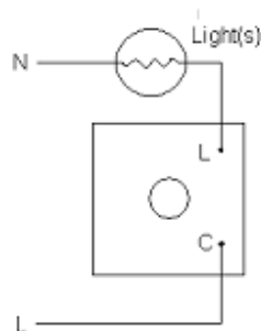
Figure 1 Using a 1-way Dimmerswitch
