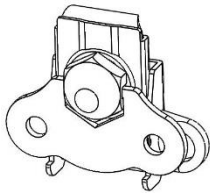
Butterfly Latch (2 Supplied)
