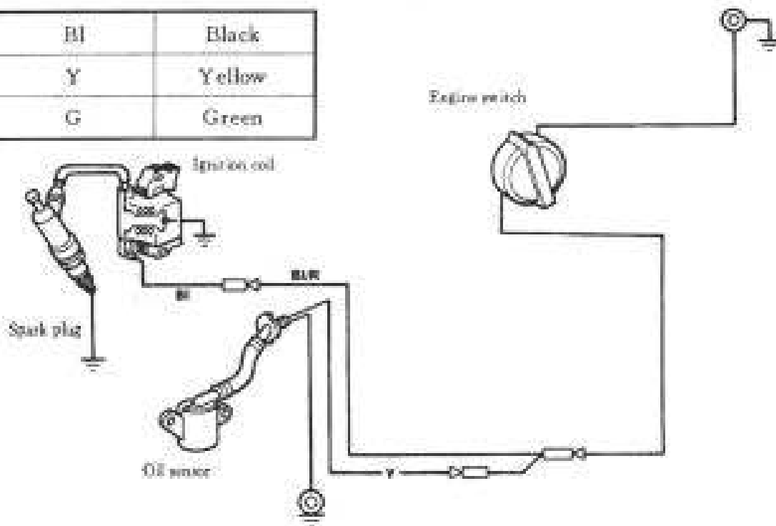
ELECTRIC DIAGRAM
