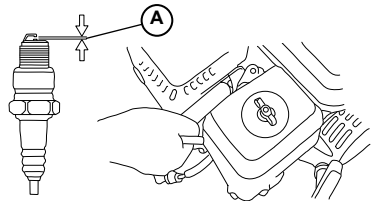
Figure 4-8. Spark Plug
