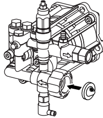
Figure 2-10. Inspect Inlet Screen
