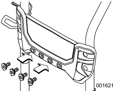
Figure 2-5. Insertion des buses
