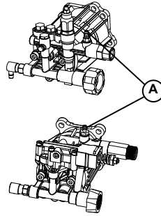
Figure 2-6. Attach Siphon Tube
