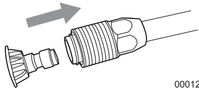
Figure 2-17. Insertion de la buse
