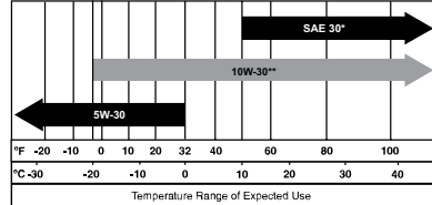
Figure 4-4. Oil Viscosity
