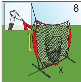
8. Grip the pole and slide the sleeve up before looping the white rope around the metal pole top.
