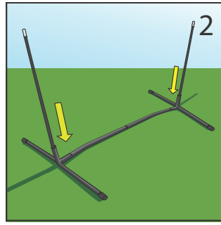
2. Install the two lower fiberglass poles, with coupling tubes at the top, into the angled pipes on the metal base.
