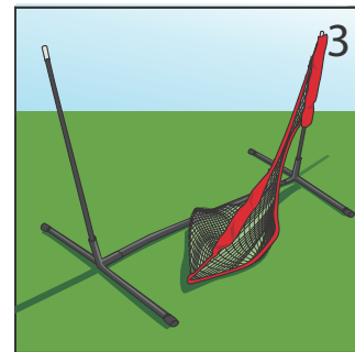
3. Thread a fiberglass pole through one of the net's sleeves making sure the net is right side up (white loops at the top corners and black bungees at the bottom corners).
