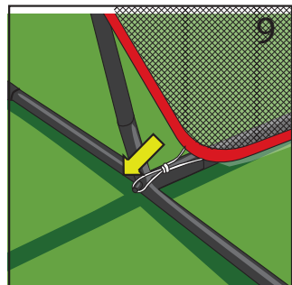
9. Loop the black elastic bungees over the metal posts located on the outside of each end leg. 10. Wrap the velcro around the frame (X in Fig. 8).
