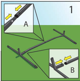
1. Join the two slightly bent pipes together (Fig. A) Then attach both end legs (Fig. B)
