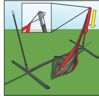
3. Thread one sleeve over a fiberglass rod and loop the white cord over the top of the rod.
