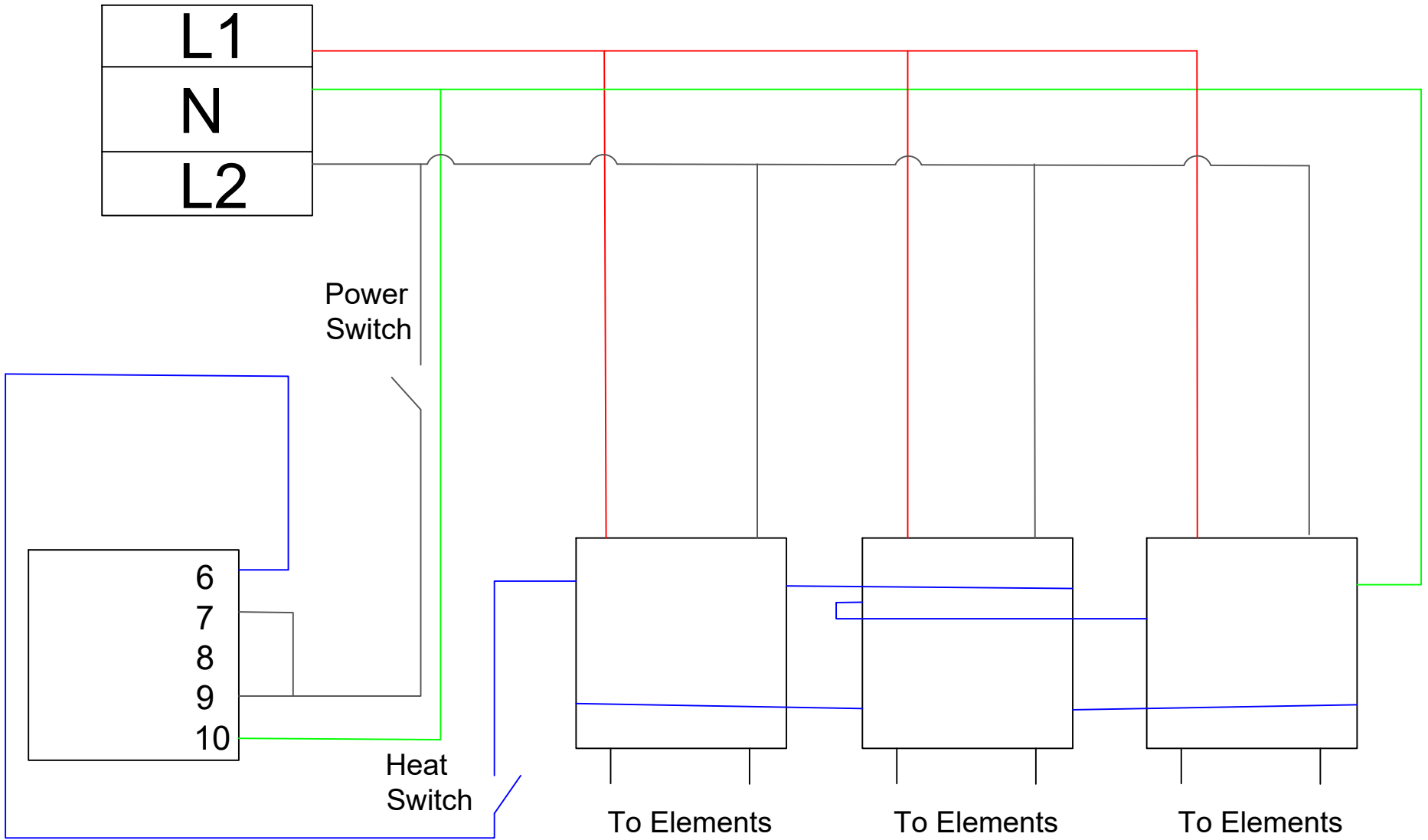
240V Single Phase, Triple Contactor
