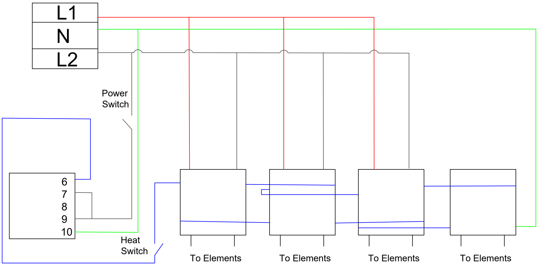
240V Single Phase, Four Contactor
