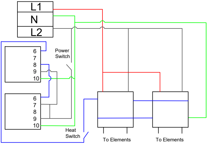
240V Single Phase, Double Contactor TIMER
