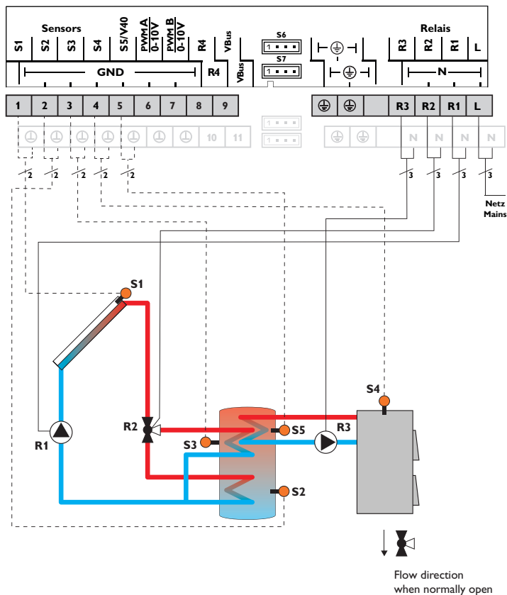
Hydraulic variant 1
