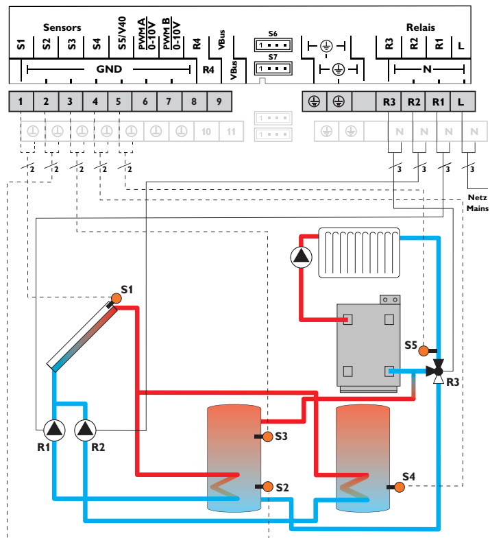
Hydraulic variant 1
