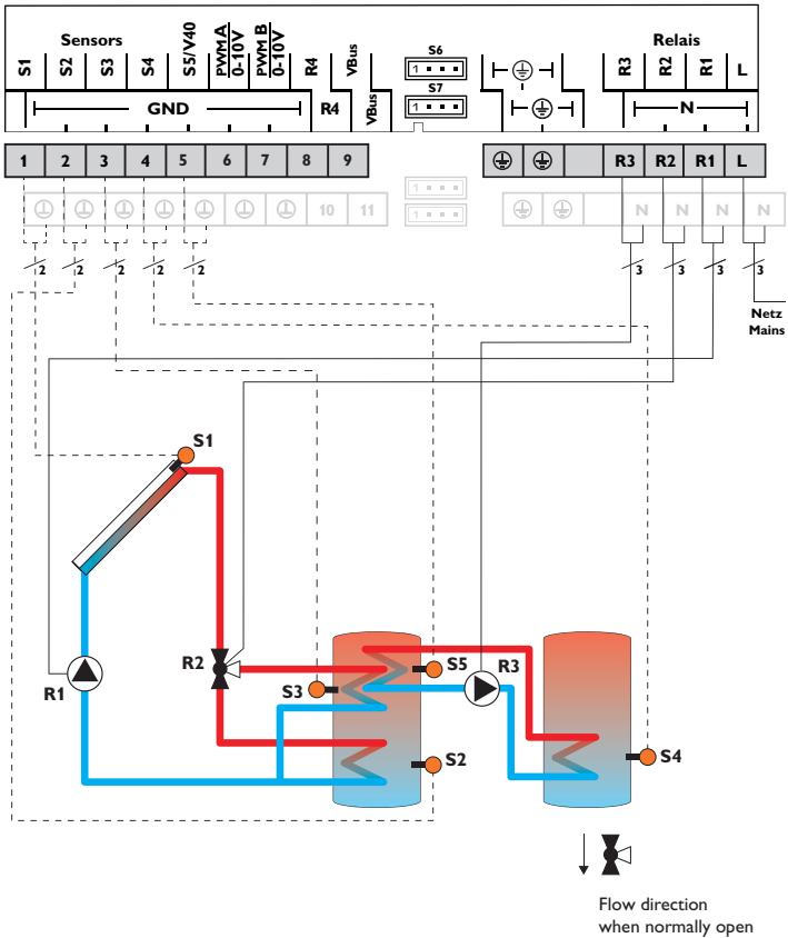
Hydraulic variant 1
