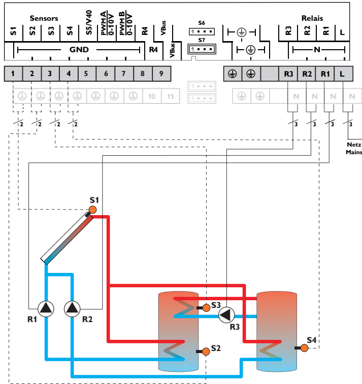
Hydraulic variant 1
