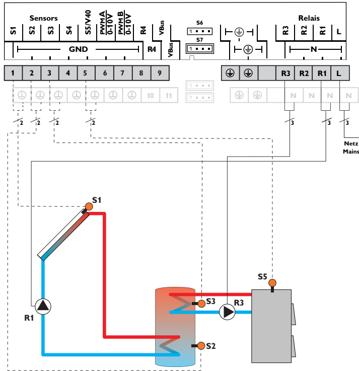
Hydraulic variant 1
