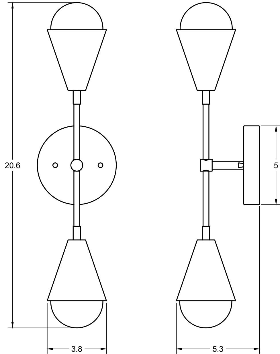
SHOP DRAWINGS
