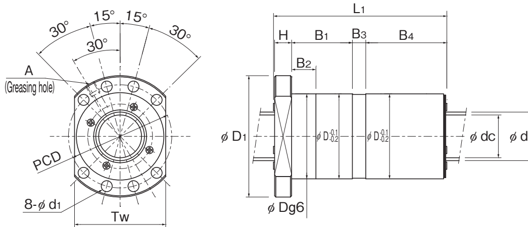
SDAN36V to 50V
