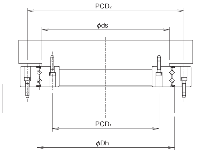
Model RW (U Type) With seal (outer-ring counterbore side)
