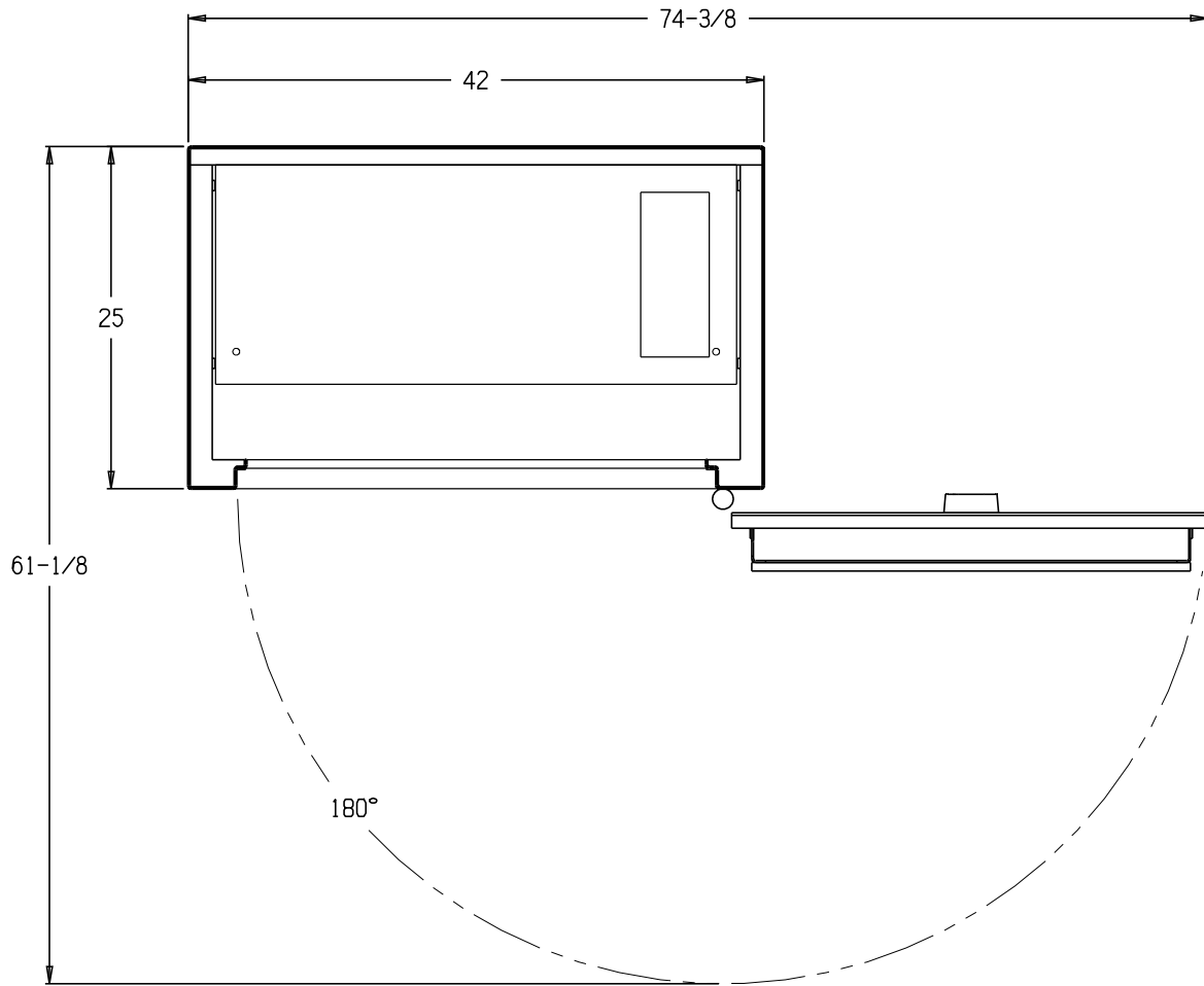
PLAN SECTION VIEW TOP SHELF
