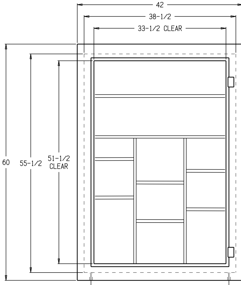
FRONT VIEW (SHOWN WITHOUT DOOR)
