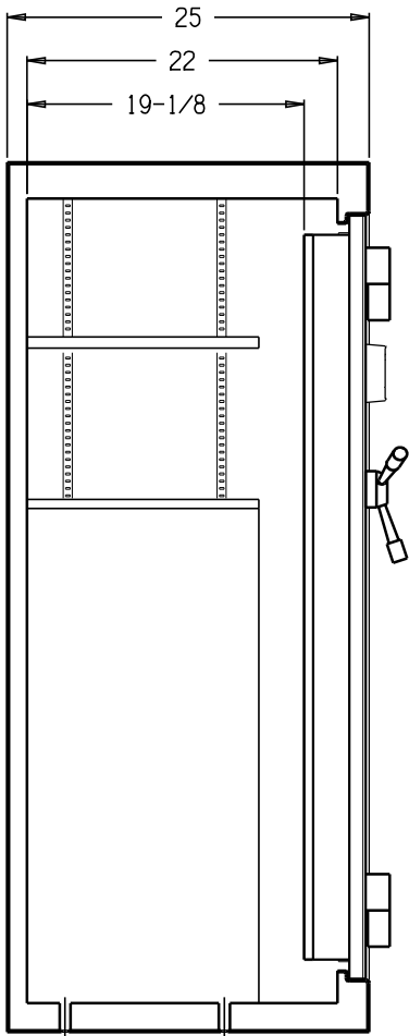
SECTION VIEW
