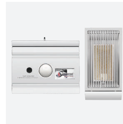
SEAR SIDE BURNER SSEAR-1 Total BTUs: 26,000 Infrared Burner (Up to 1600°F) Adjustable High/Low Technology Cooking Surface: 18 1 / 2 x 11 1 / 2
