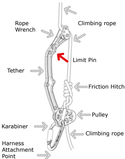
Fig 2 Fully Assembled Rope Wrench System
