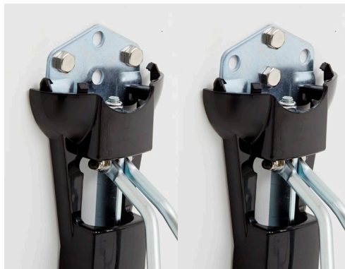
Bolt positions for masonry
