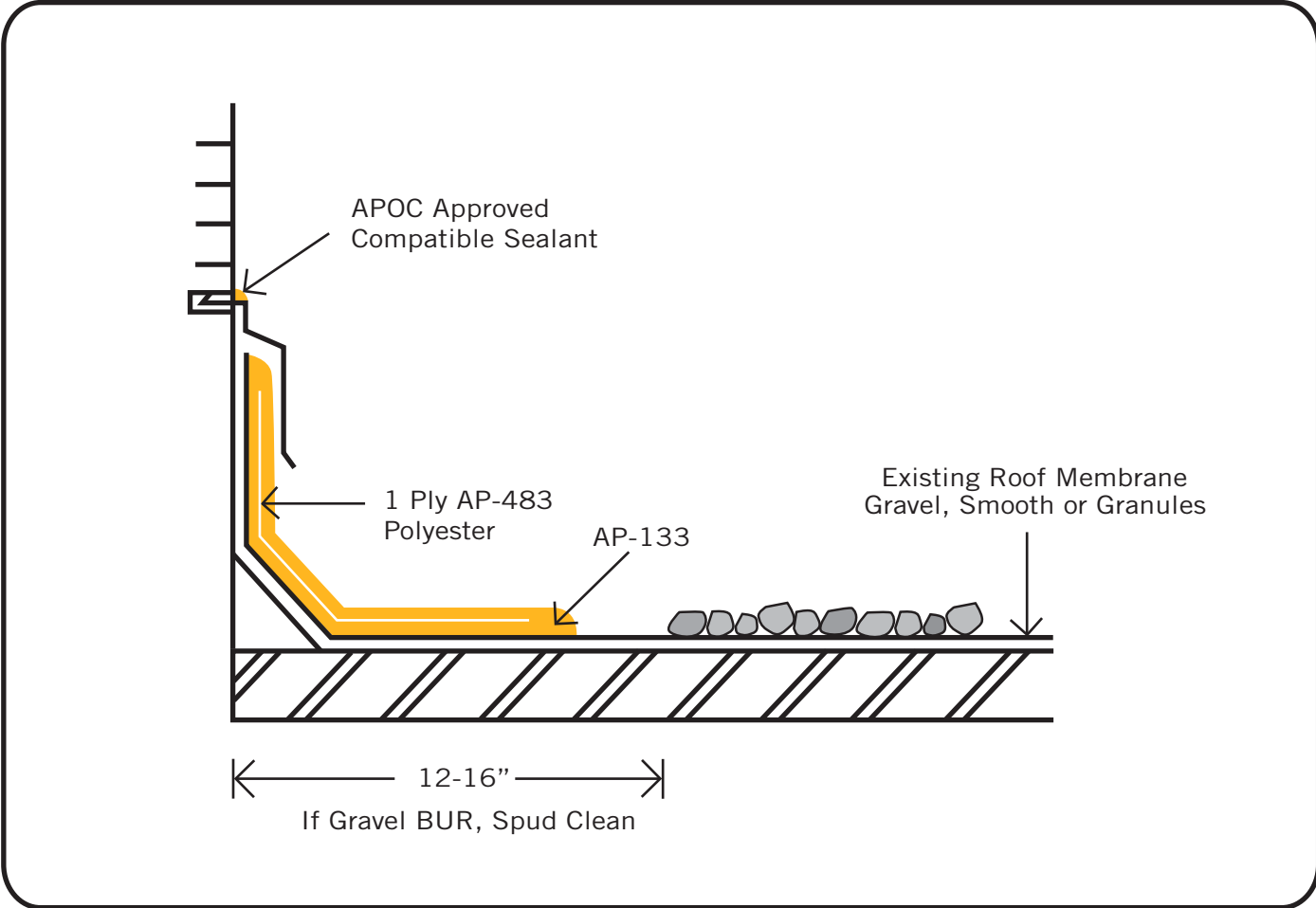
Detail: BUR-8-Asphalt Base Flashing w/Saw Cut Repair
