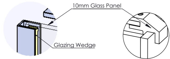
Glass to Wall Tolerance DETAIL A
