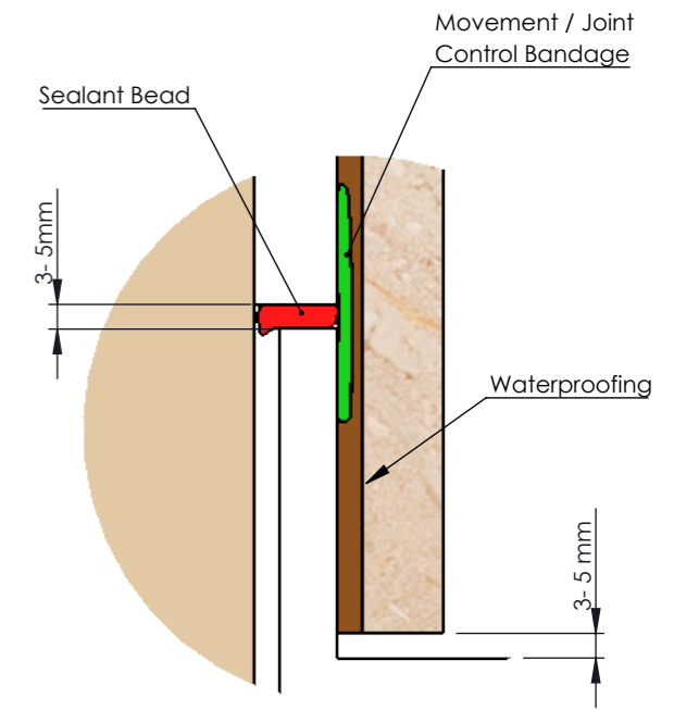
Wall Joint Detail DETAIL C
