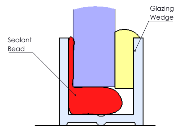
Glass Panel Silicone Detail DETAIL D
