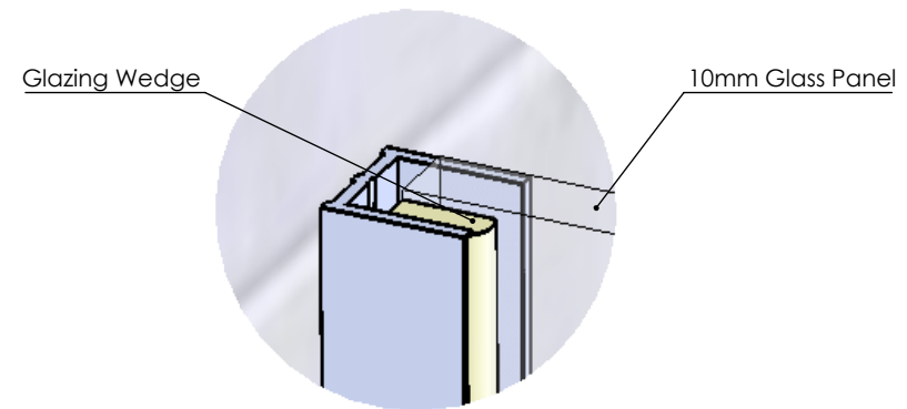
Glass To Wall Tolerance DETAIL A
