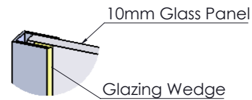
Glass To Wall Tolerance DETAIL A
