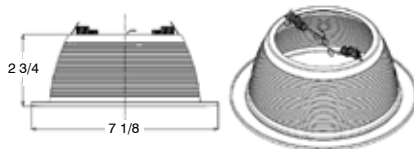
RT601BL/WH Black Step Baffle with White Ring Uses BR/PAR30 Lamps Order Code: 77102
