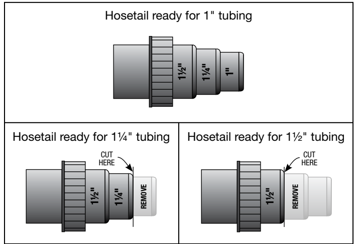
UltraKlear® with Rotational Ball Fittings and Multi-Hose Adapters
