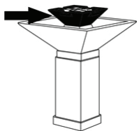
FT-348B (11 lbs) 10.5"L x 10.5"W x 3.75"H
