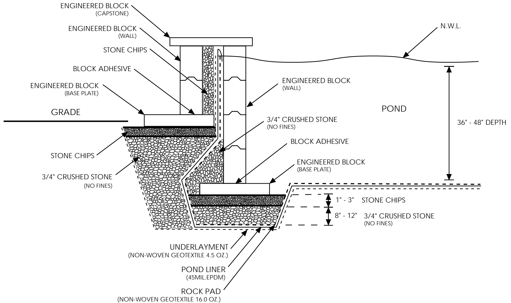
SIDE VIEW DETAIL
