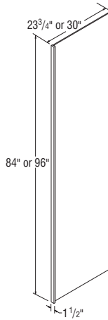
PREPRP1.584* PREPRP1.596* PREPR1.53084* New PREPR1.53096* New
