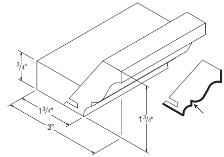
Full Overlay MFOLCR8 (1 - 8' pc) PSMFOLCR8 (1 - 8' pc)
