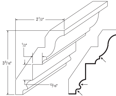
Insert MICROWN8 (1 - 8' pc) PSMICROWN8 (1 - 8' pc)
