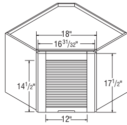
Diagonal AC2417.5
