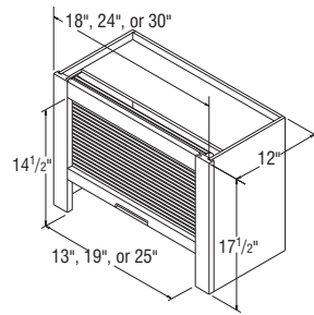
Straight ACS1817.5 ACS2417.5 ACS3017.5
