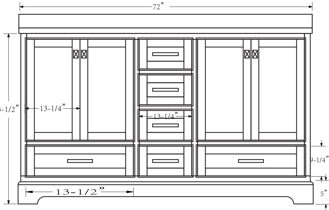
FRONT VIEW
