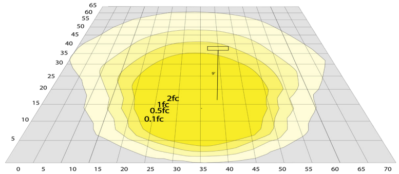
Area 65'x 70' Mounting Height: 9'
