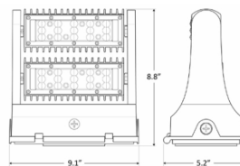
8.8" (H) x 5.2" (W) x 9.1" (L)
