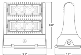
8.8" (H) x 5.2" (W) x 9.1" (L)
