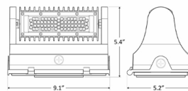
5.4" (H) x 5.2" (W) x 9.1" (L)
