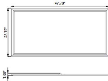
47.70"(L)X23.70"(W)X1.09"(H)
