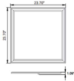
23.70"(L)X23.70"(W)X1.09"(H)
