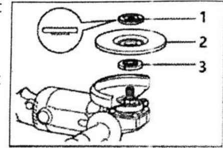
2.Depressed center grinding wheel/Multi-disc 3.Inner flange
