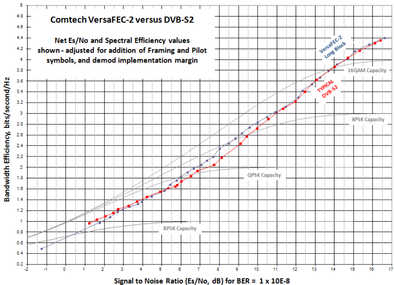
Figure 1: VersaFEC-2 vs. DVB-S2
