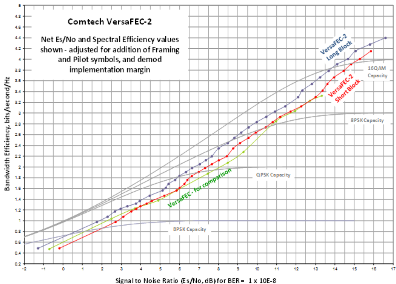
Figure 2: VersaFEC-2 vs. VersaFEC
