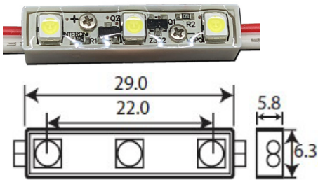
V03 Epoxy 3-LED
