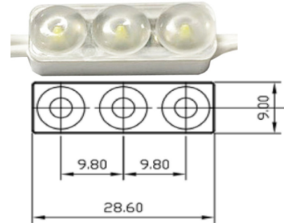
V05 Lens 3-LED
