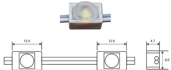
V05 Lens 1-LED
