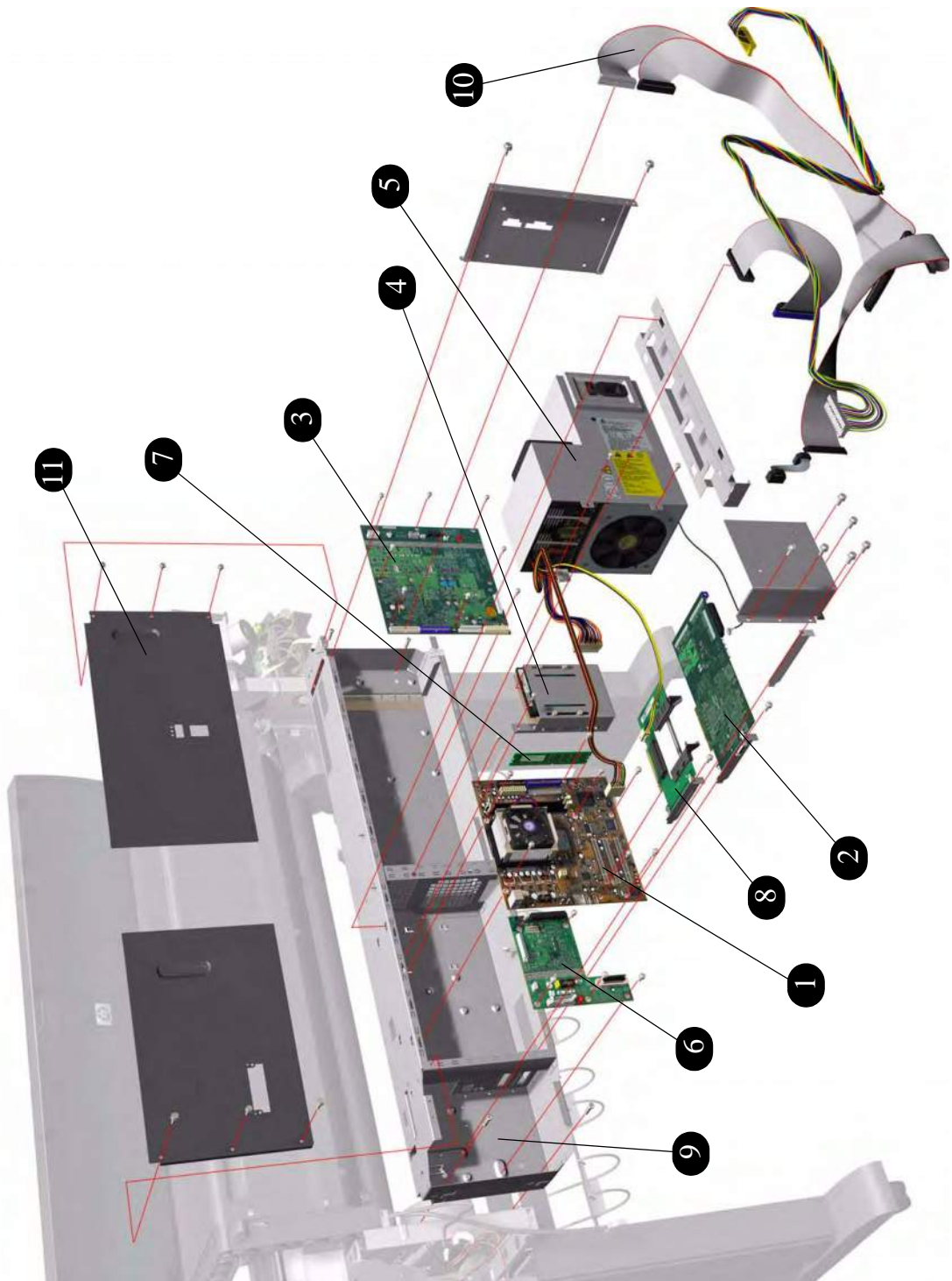
Figure 3: Electronics Module
