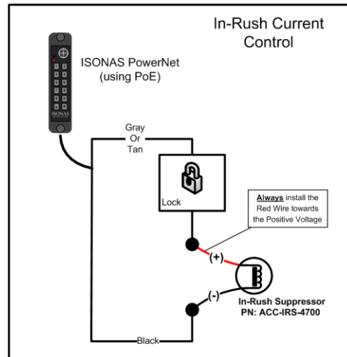
Figure 20b (ACC-IRS-4700 w/red & black wires)
