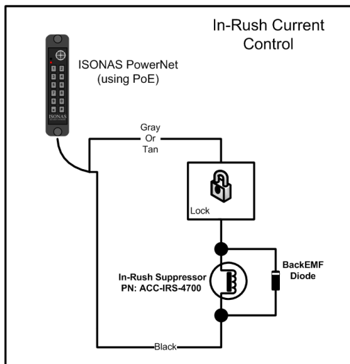
Figure 20a (ACC-IRS-4700 w/two black wires)
