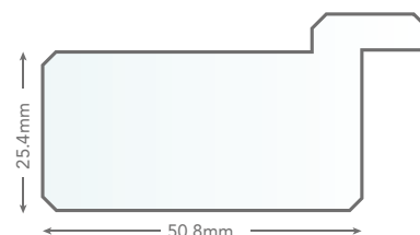
50.8mm Flat D-Mould Stile
