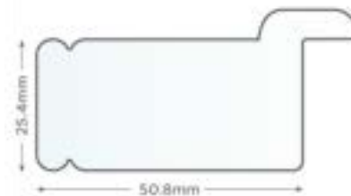
50.8mm Beaded D-Mould Stile
