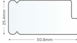
50.8mm Beaded Rebate Stile
