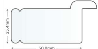
50.8mm Beaded D-Mould Stile
