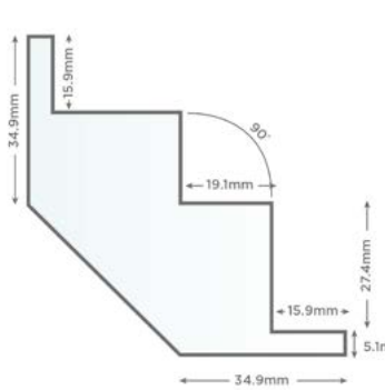
(Deco Frame) 32mm
